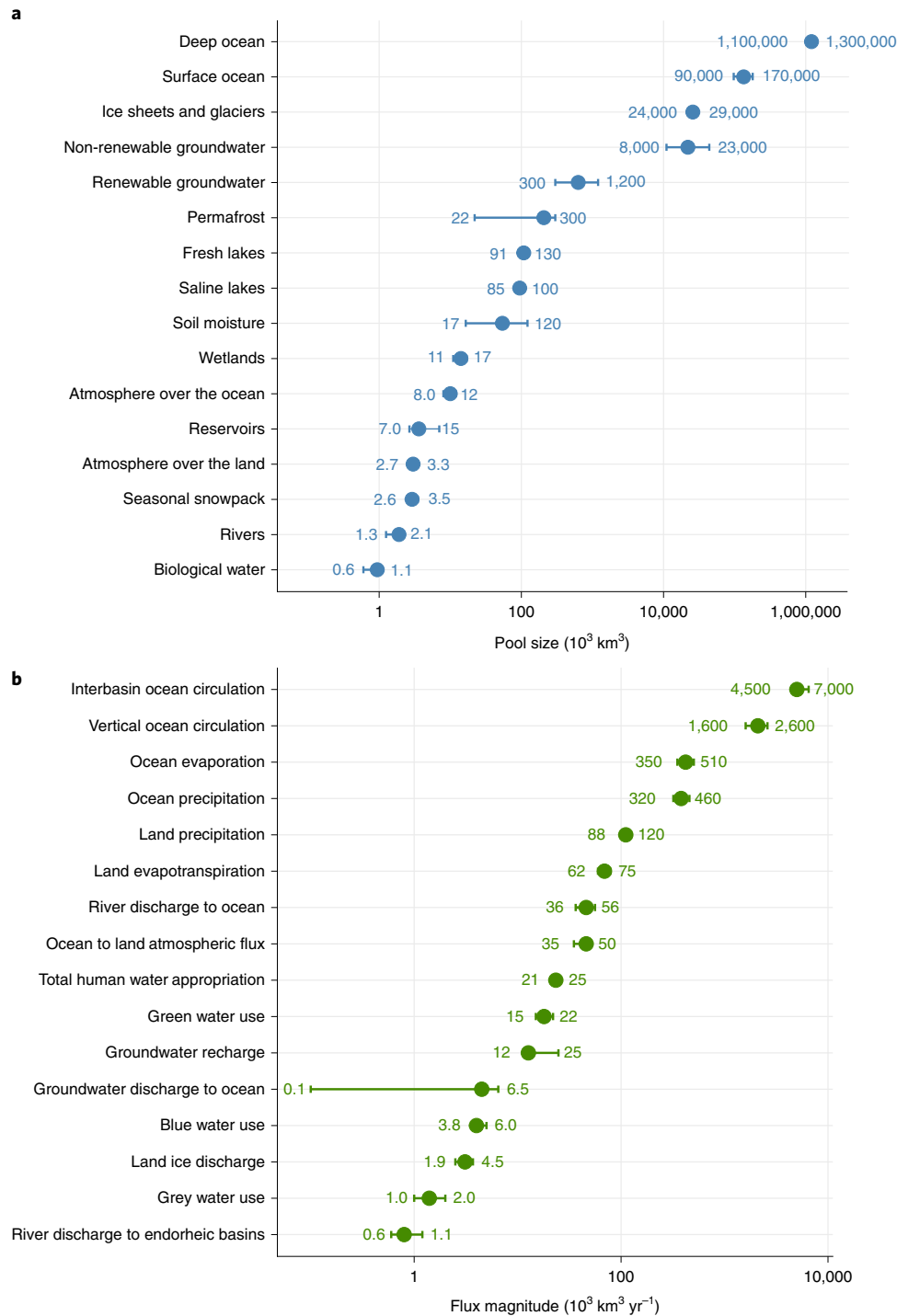
Fig. 1 | Pools and fluxes in the global hydrological cycle. a,b , Estimates of major pools ( a ) and fluxes ( b ) are based on a synthesis of ~80 recent regional- and global-scale studies (Supplementary Table 1). The central point represents the most recent or comprehensive individual estimate, and error bars represent the range of reported values and their uncertainties. Note the log scales on the x axes.
