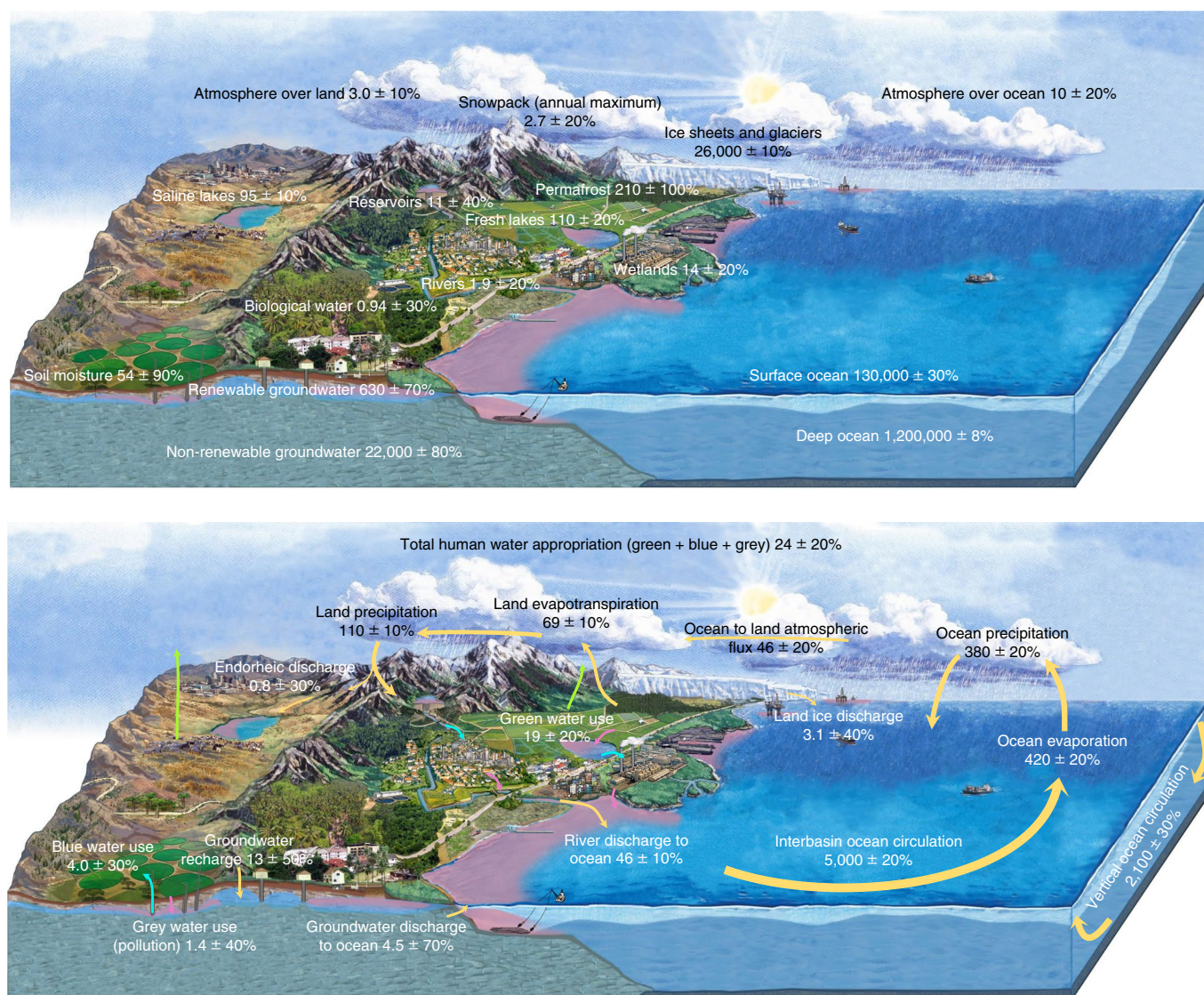
Fig. 3 | Diagram of the global hydrological cycle in the Anthropocene. a,b , Major water pools (expressed in 10^3 \text{ km}^3 ) (a) and water fluxes (expressed in 10^3 \text{ km}^3 \text{ yr}^{-1} ) (b). Uncertainty represents the range of recent estimates expressed in %. In b , we separate total human water use ( \sim 24 \times 10^3 \text{ km}^3 \text{ yr}^{-1} ) into green (soil moisture used by human crops and rangelands, green arrows); blue (consumptive water use by agriculture, industry and domestic activity, blue arrows); and grey (water necessary to dilute human pollutants, which is represented with pink shading, pink arrows). This averaged depiction of the hydrological cycle does not represent important seasonal and interannual variation in many pools and fluxes.
