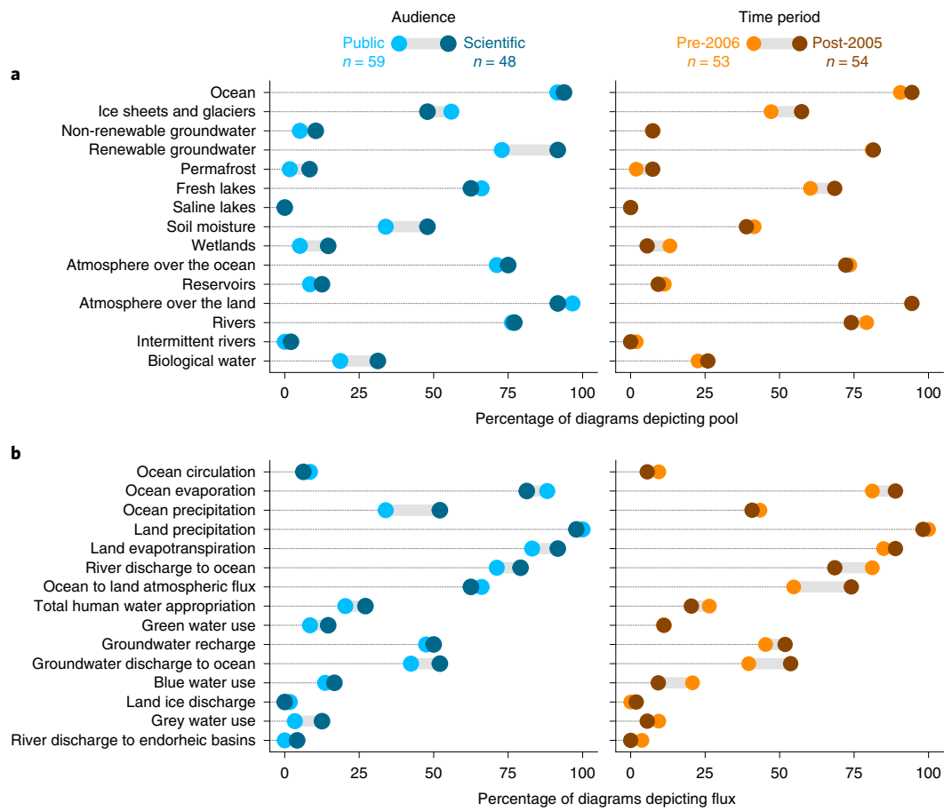
Fig. 2 | Pools and fluxes represented in water cycle diagrams. a, b, Percentage of water cycle diagrams that represent major pools ( a ) and fluxes ( b ) in the global water cycle. Pools and fluxes are ordered by size based on Fig. 1, starting with the largest pool (ocean) and flux (ocean circulation). We categorized diagrams by intended audience and time period. Public diagrams include those made for advertising, advocacy, government outreach and primary or secondary education, whereas scientific diagrams were made for higher education textbooks and peer-reviewed publications. We compared the diagrams made before and after 1 January 2006, which corresponds with the publishing of several high-profile papers that advocated increased integration of social and hydrological systems. The grey bar between points is visible for differences greater than 10 percentage points.
